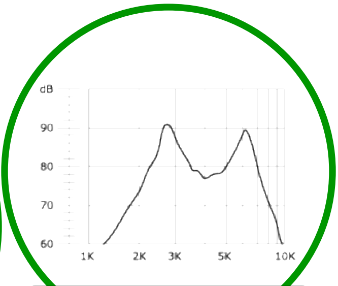
Frequency Response Measuring Temperature : 25°C Measuring Distance : 10cm
