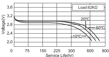
Temperature Characteristics
