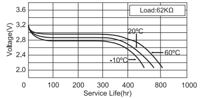
Temperature Characteristics
