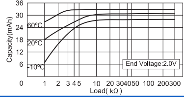
Pulse Discharge Characteristics
