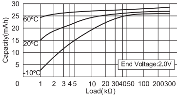
Pulse Discharge Characteristics
