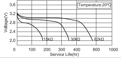
Load-capacity
