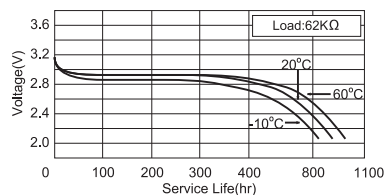
Temperature Characteristics
