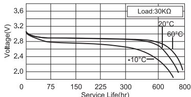
Temperature Characteristics
