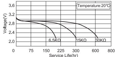
Load-capacity
