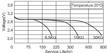
Load-capacity
