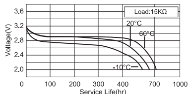
Temperature Characteristics
