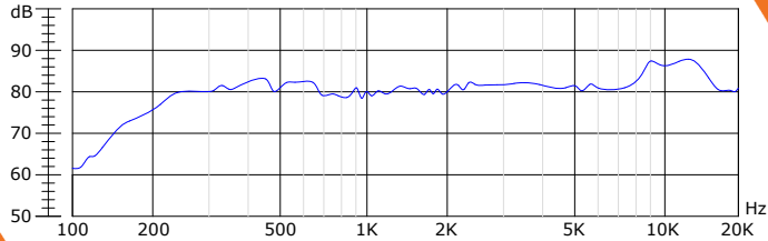
Frequency Response Normalized to 1W Input Power and 0.5m Measuring Distance
