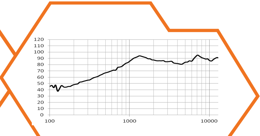
Frequency Response Normalized to 0.5W Input Power and 0.3m Measuring Distance
